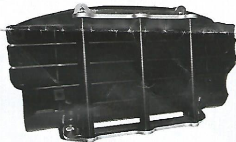
Fix the bloc M6x16 + M6x20 on the air deflector points
